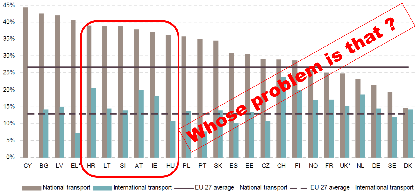
Figure 7: Share of empty vehicle-kilometres in the total vehicle-kilometres by type of operation, 2010 (% on vkm)
